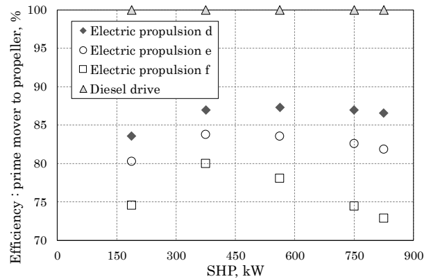
Fig.5 Estimated results of total efficiency from prime mover or AC line to propeller as diesel drive system's efficiency is 100%
