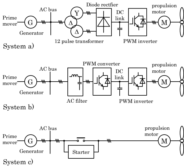
Fig.1 Electric propulsion system with AC bus
