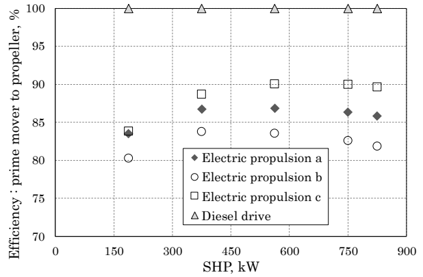
Fig.2 Estimated results of total efficiency from prime mover to propeller as diesel drive system's efficiency is 100%
