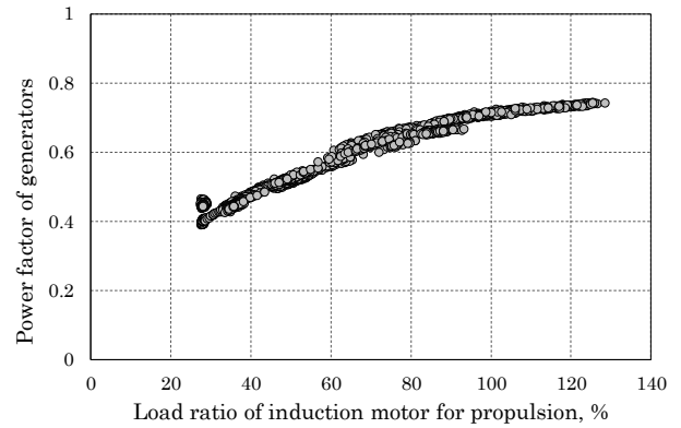
Fig.3 Sample of power factor to load ratio of propulsion motor measured by system c) in actual
